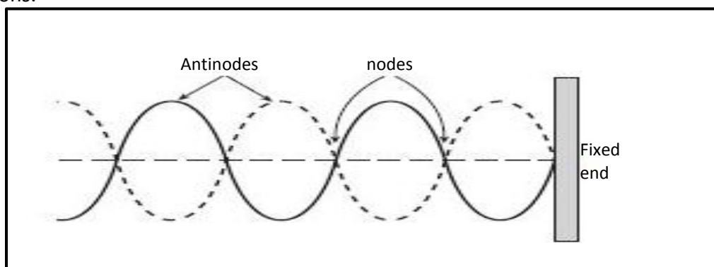
Figure 21: A standing wave produced by the continual generation and reflection of waves off a fixed wall. Oscillation only occurs between the dashed and solid lines.
