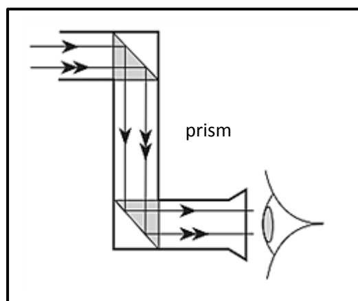
Figure 48b: Periscopes use total internal reflection in prisms.
